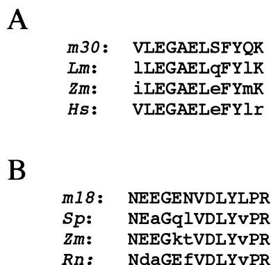
Fig. 4. Alignment of m30 and m18 peptides with matching ribosomal subunit proteins S8 (A) and S21 (B), respectively. Mismatches are in lower case letters. Lm : Leishmania major , SwissProt accession number P25204; Zm : Zea mays , SwissProt accession number Q08069 (panel A) and EMBL accession number Y09636.1 (panel B); Hs : Homo sapiens [25]; Sp : Schizosaccharomyces pombe , SwissProt accession number P05764; Rn : Rattus norvegicus , SwissProt accession number P05765.
